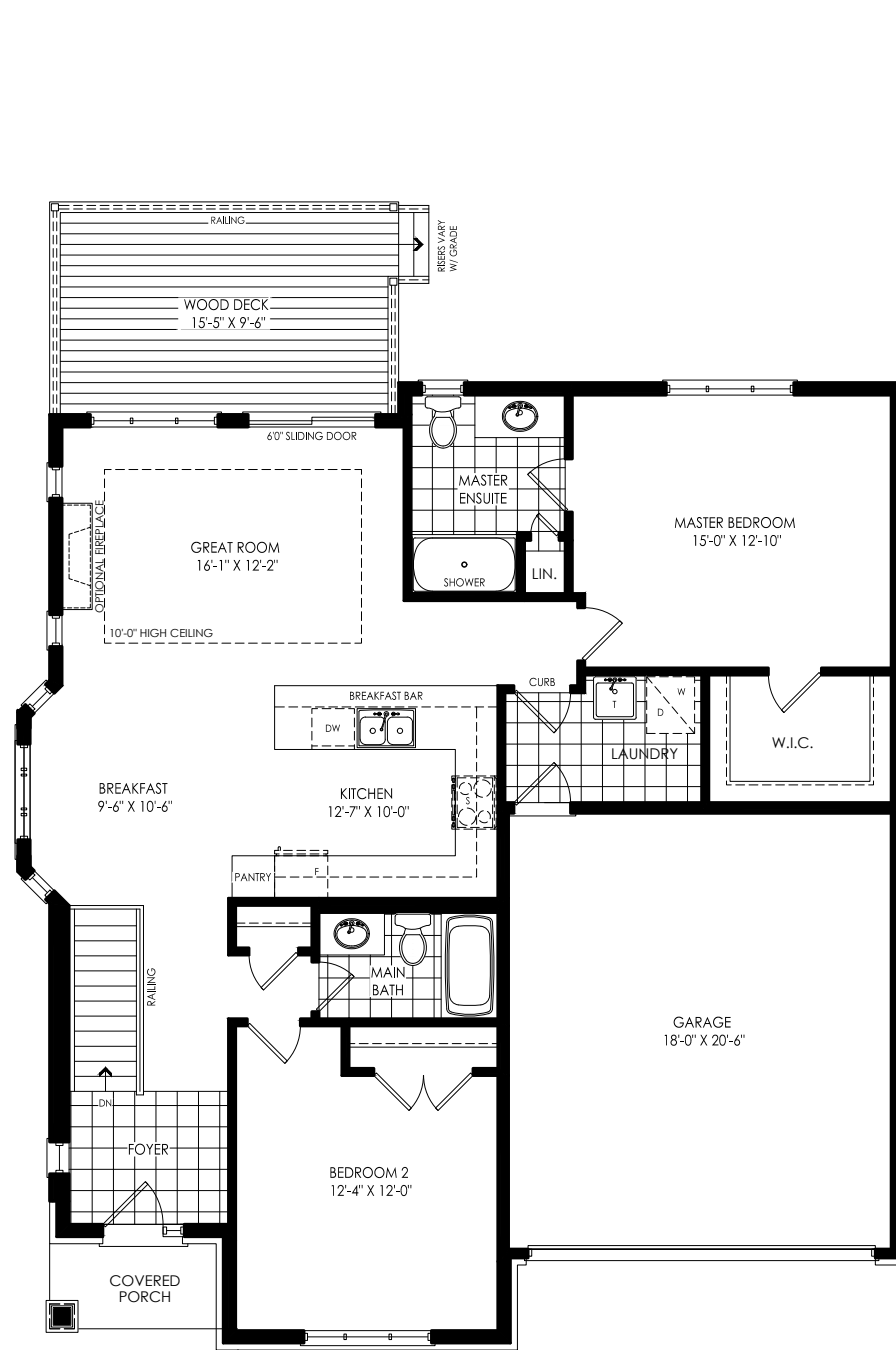
GROUND FLOOR
