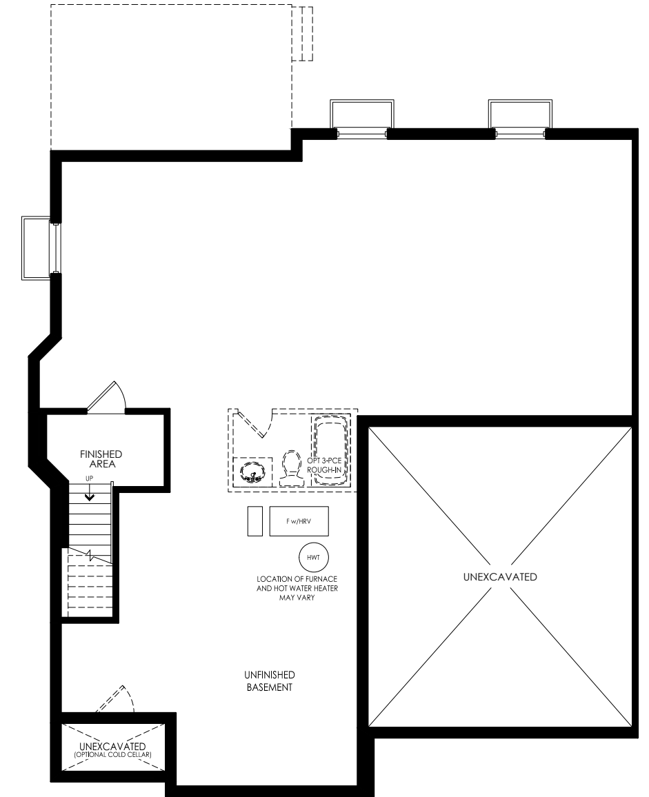
BASEMENT FLOOR
